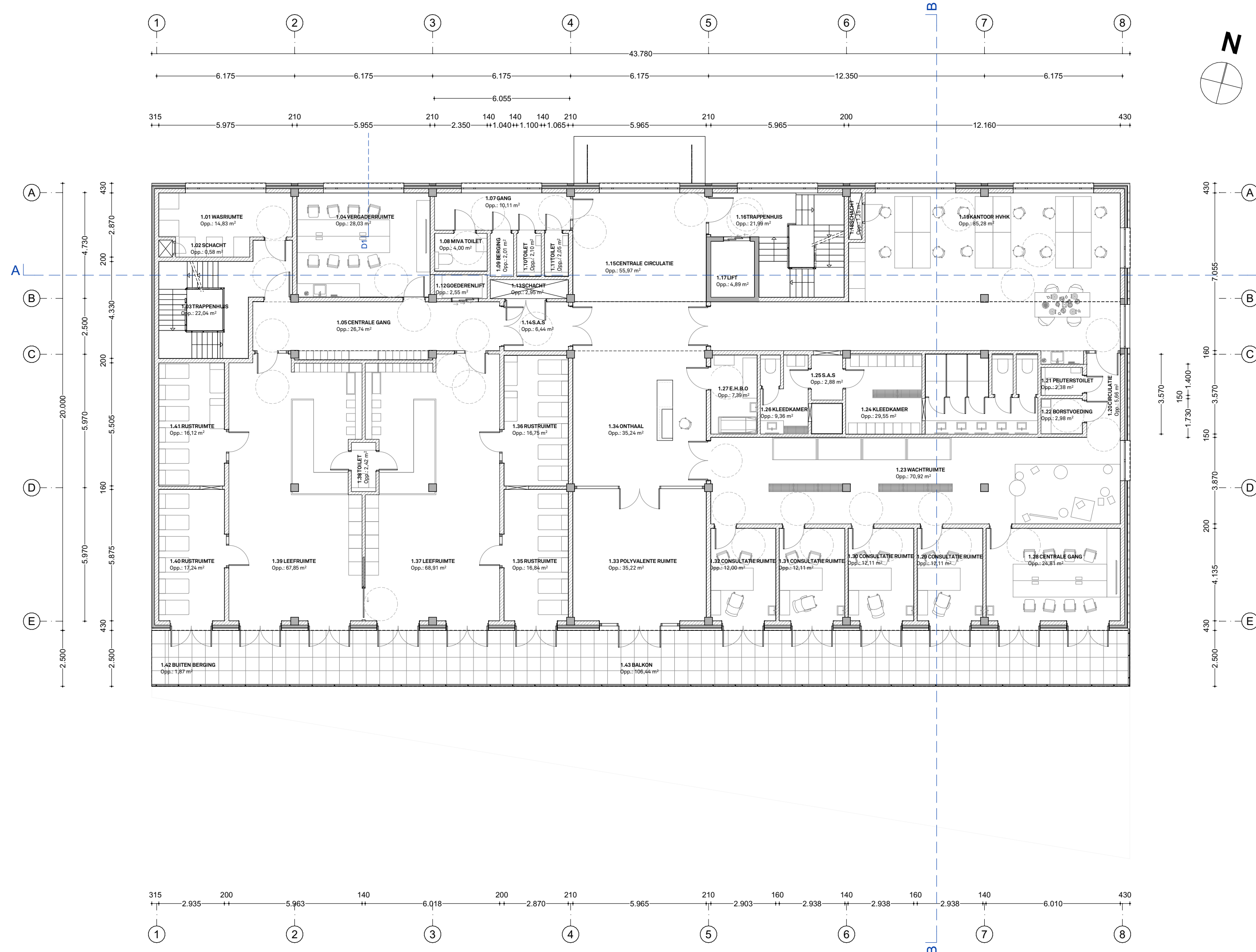
PLAN +1
