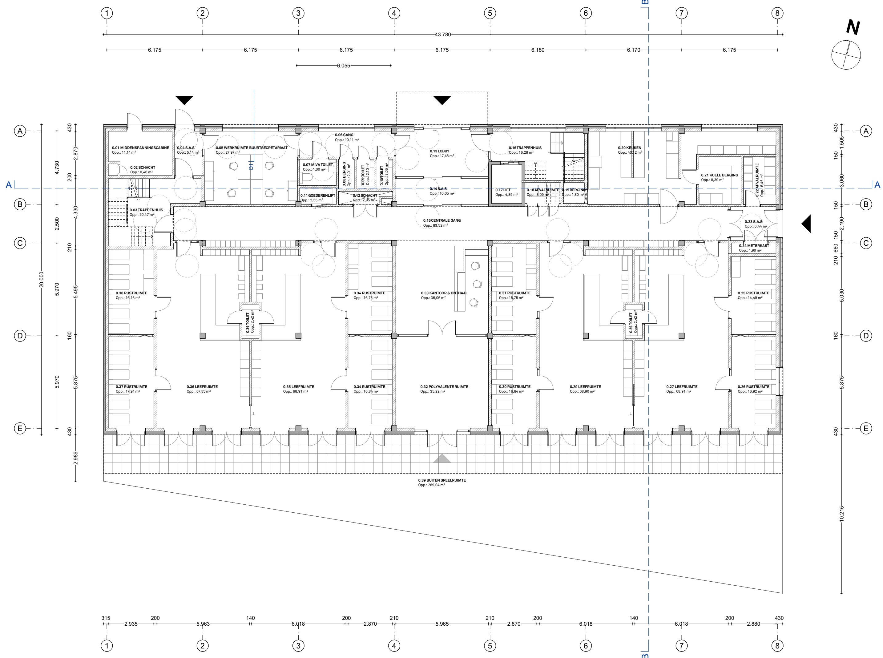
PLAN +0
